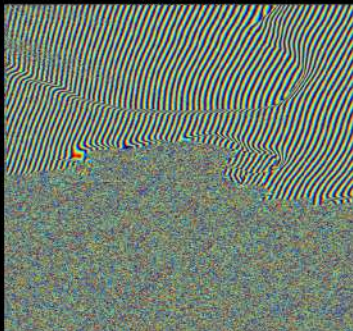
Interferogram phase 2026-05-01~2026-05-04
