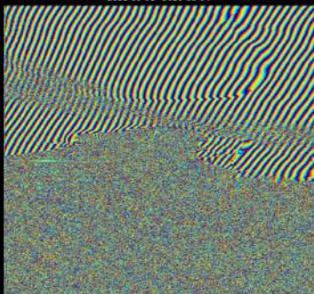
Interferogram phase 2026-05-04~2026-05-07
