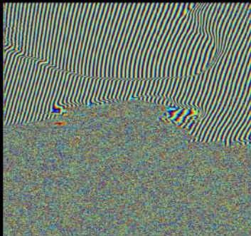
Interferogram phase 2026-04-28~2026-05-01
