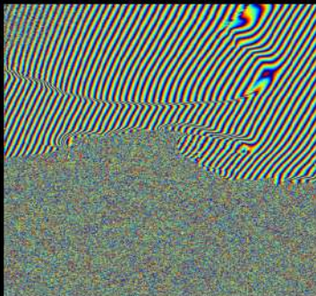
Interferogram phase 2026-05-10~2026-05-13
