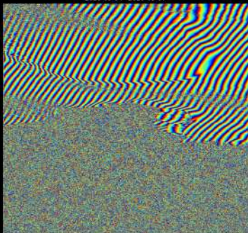
Interferogram phase 2026-05-07~2026-05-10
