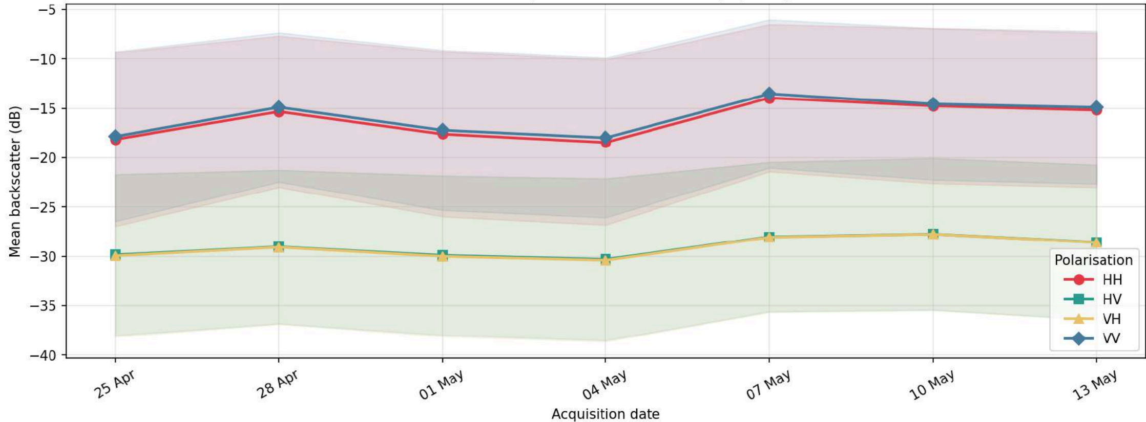
Temporal backscatter — Antarctic Ice Shelf Biomass L1a P-band | Track T034 Frame F250 | Apr-May 2026
